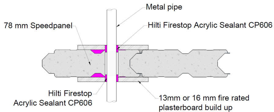
Figure 3 Horizontal cross section for build-up and sealant in Speedpanel/Speedwall
