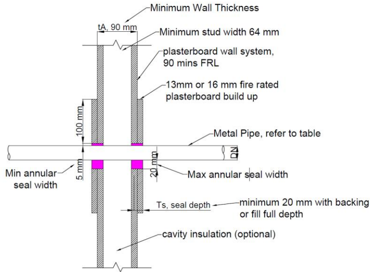
Figure 10 Side view – 1hr FRL single layer plasterboard with sealant and plasterboard build-up
