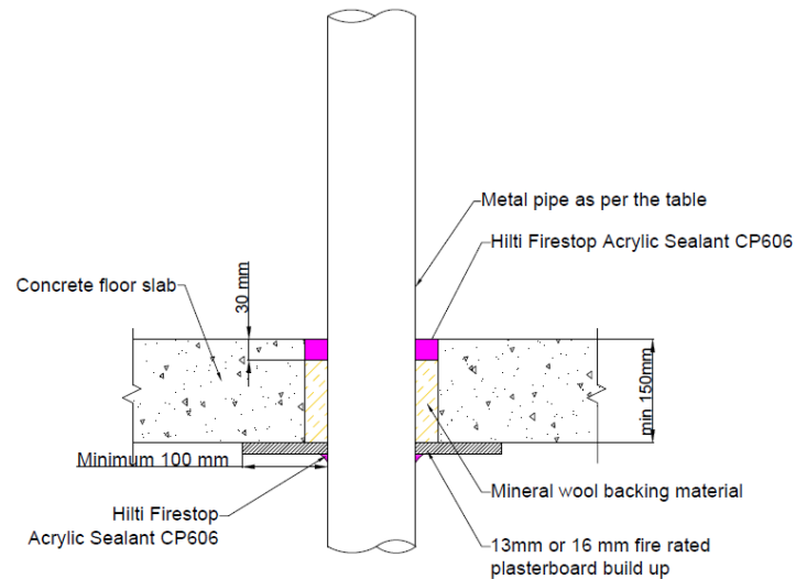
Figure 7 Larger annular gaps in floor configurations
