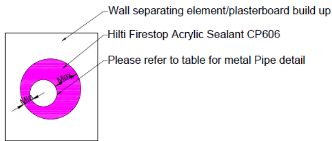
Figure 20 Front view – annular gap
