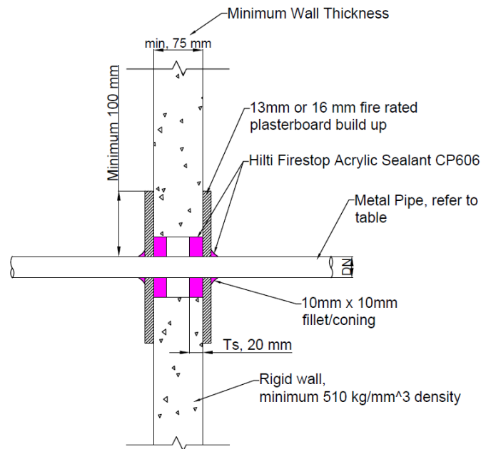
Figure 6 Larger annular gaps in wall configurations
