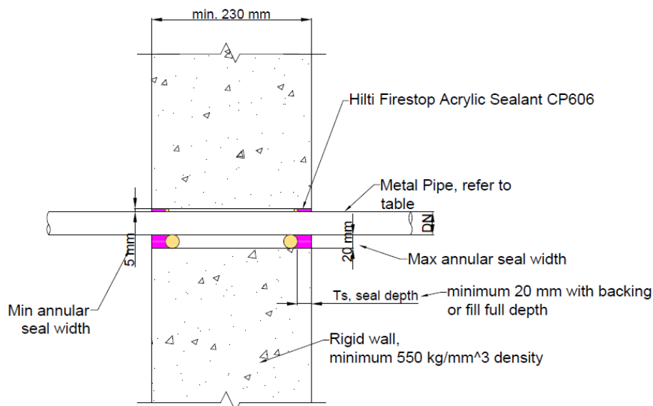
Figure 23 Side view – 240 mins FRL rigid wall system with sealant only
