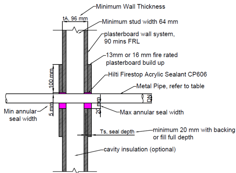
Figure 13 Side view – 90 mins FRL plasterboard system with sealant and plasterboard build-up
