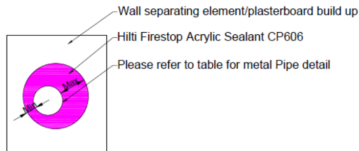
Figure 12 Front view – Annular Gap
