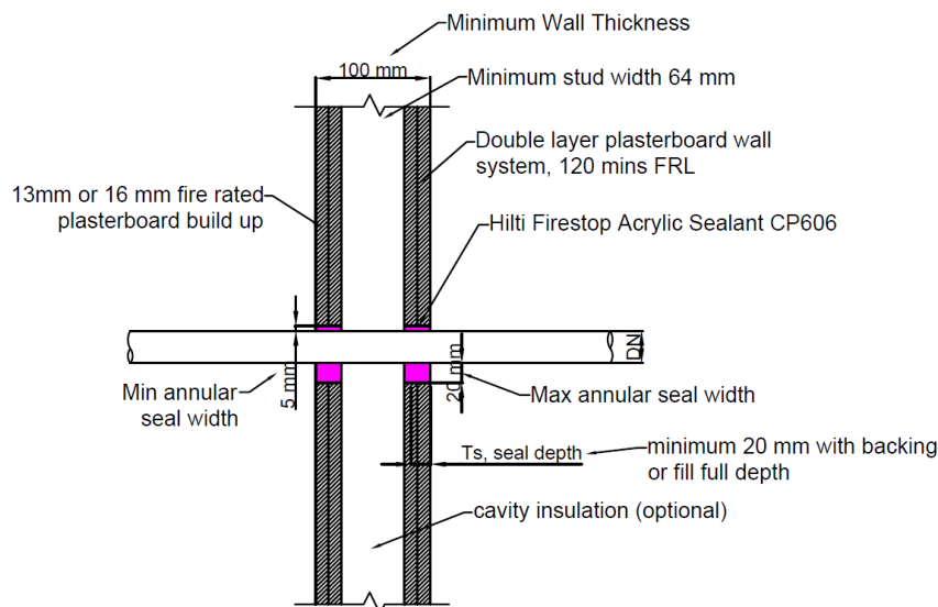
Figure 16 Side view – 120 mins FRL plasterboard system with sealant only
