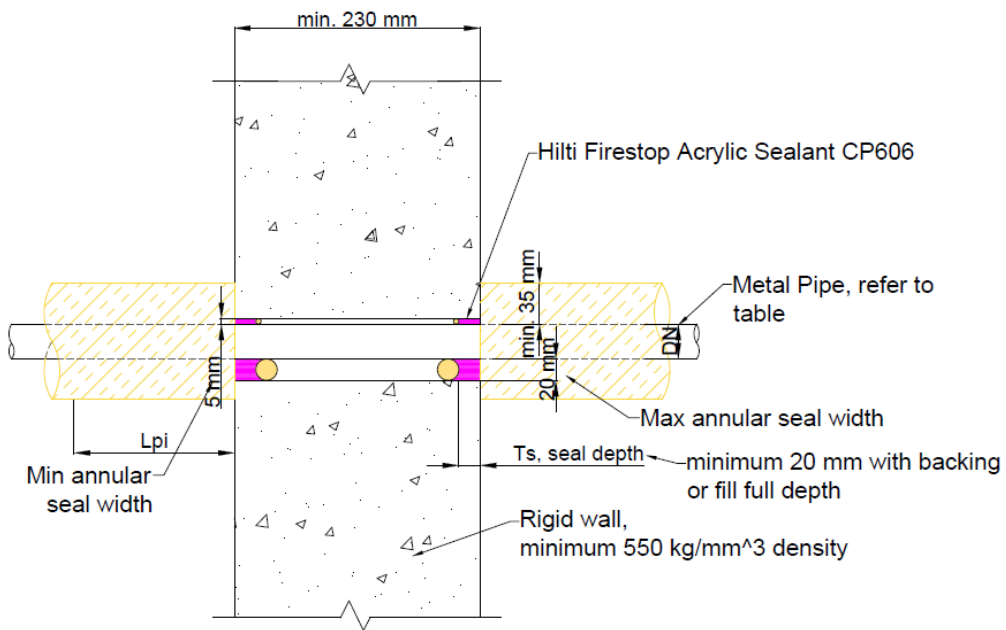
Figure 24 Side view – 240 mins FRL rigid wall system with sealant and mineral wool insulation
