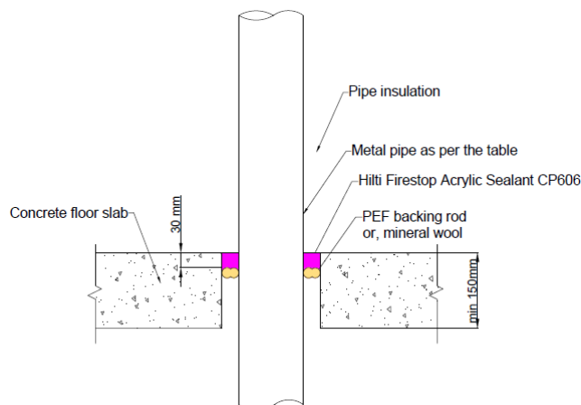
Figure 26 Side view – 120 mins FRL rigid floor system with sealant only
