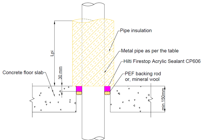
Figure 27 Side view – 120 mins FRL rigid floor system with or without mineral stone wool
