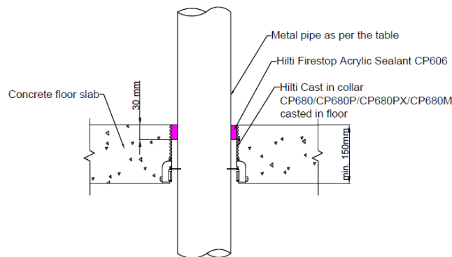
Figure 25 Side view – 120 mins FRL rigid floor with cast-in collar in concrete slab detail
