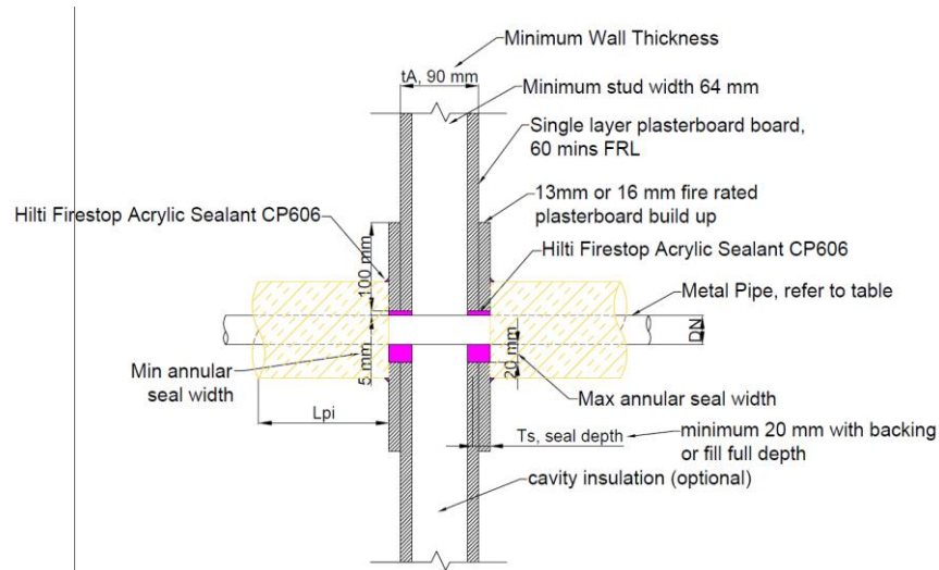
Figure 11 Side view – 1hr FRL single layer plasterboard with sealant, plasterboard build-up and mineral wool insulation
