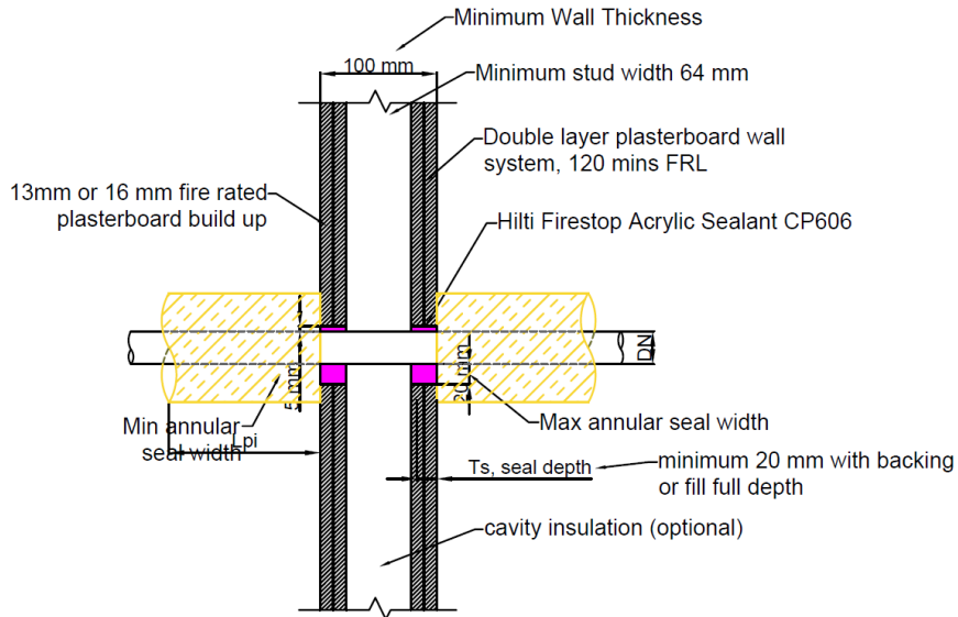
Figure 18 Side view – 120 mins FRL plasterboard system with sealant and mineral wool insulation
