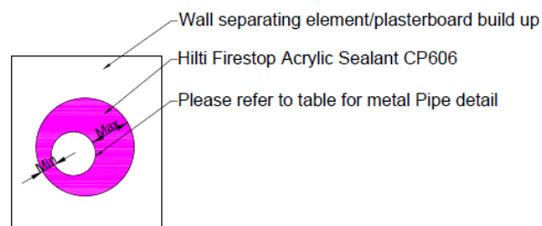
Figure 16 Side view – 120 mins FRL plasterboard system with sealant only
