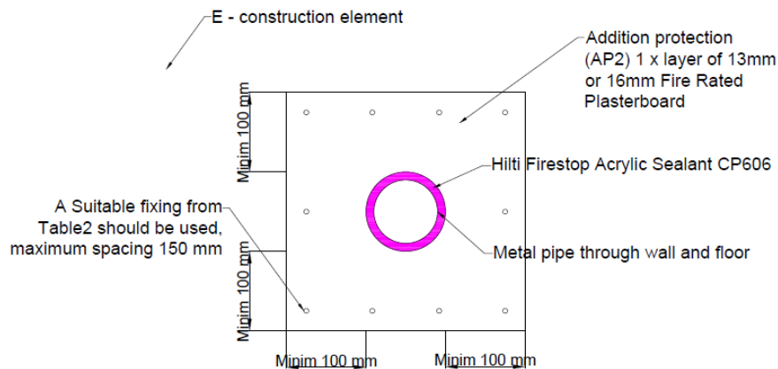
Figure 4 Elevation of aperture framing / beading and position of the seal in walls
