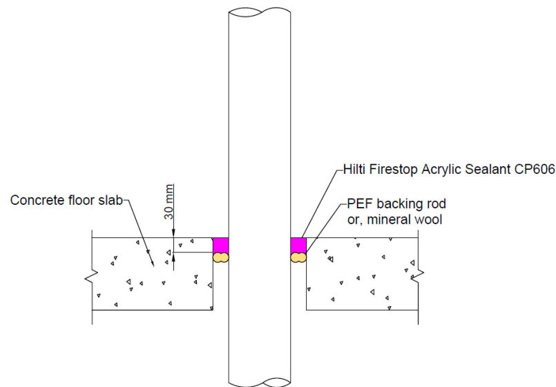
Figure 2 Generic floor penetration configuration
