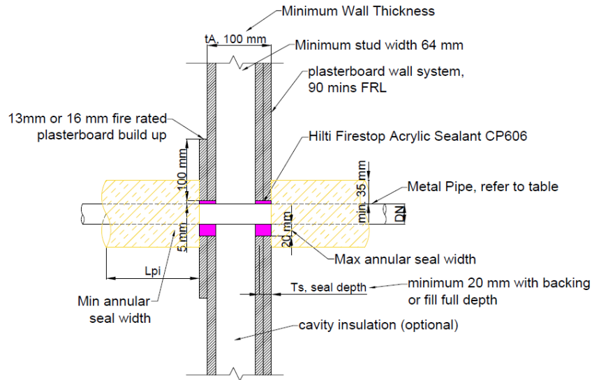
Figure 14 Side view – 90 mins FRL plasterboard system with sealant, plasterboard build-up and mineral wool insulation
