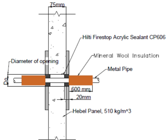
Figure 22 Side view – 120 mins FRL rigid wall system with sealant, plasterboard build-up and mineral wool insulation
