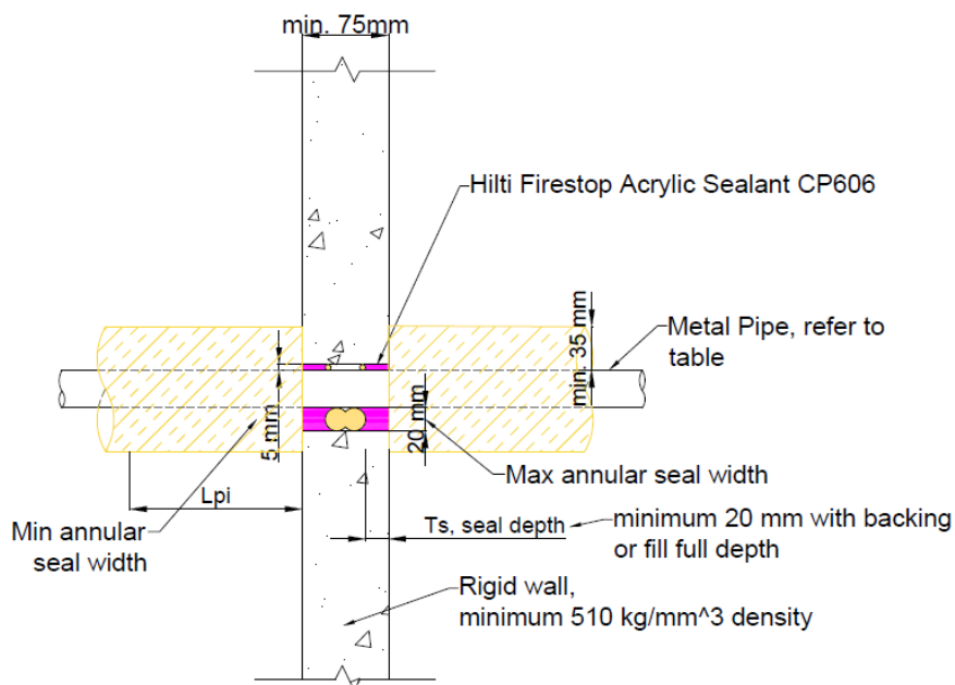
Figure 21 Side view – 120 mins FRL rigid wall system with sealant and mineral wool insulation
