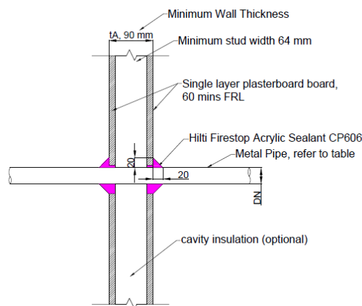
Figure 8 Side View - 1hr FRL single layer plasterboard with sealant only
