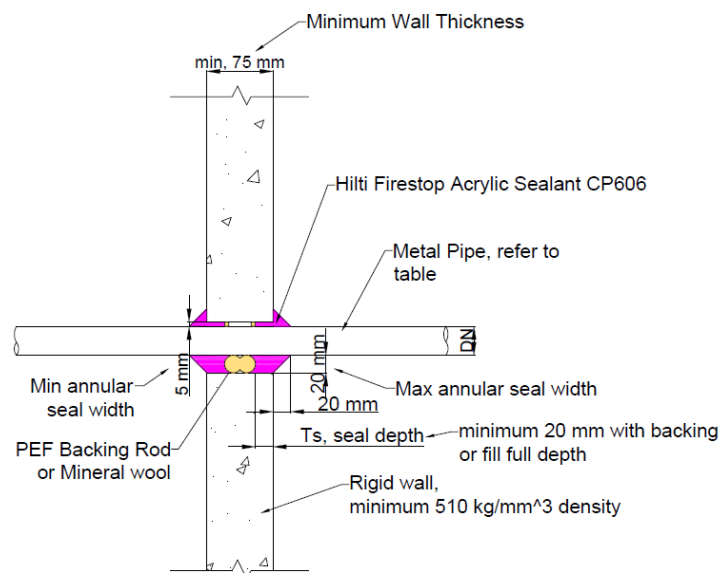
Figure 19 Side view – 120 mins FRL rigid wall system with sealant only
