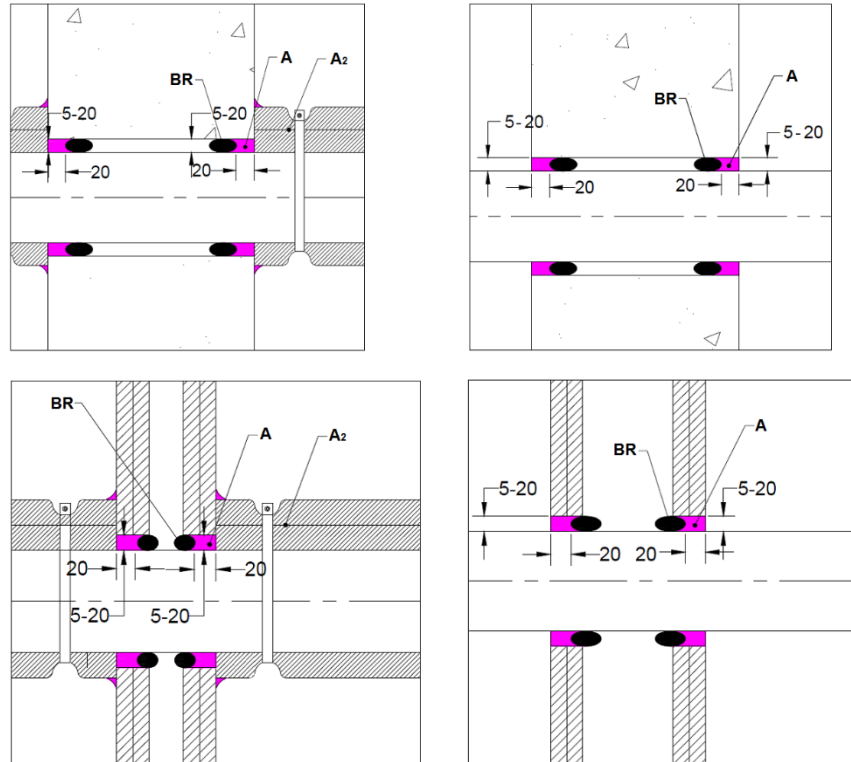
Figure 5 Sealant detail for Rigid and Flexible walls with and without pipe insulation
