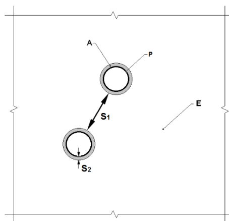
Figure 1 Distance requirements of penetrations (sealant to minimum depth of 20 mm)
